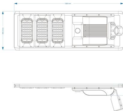
FX-50W/60W
