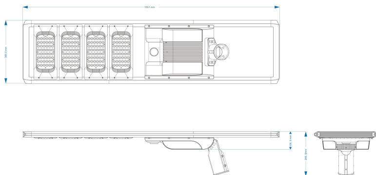
FX-50W/60W
